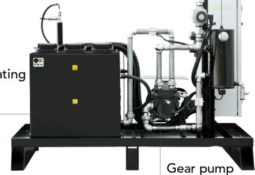
Gear pump
